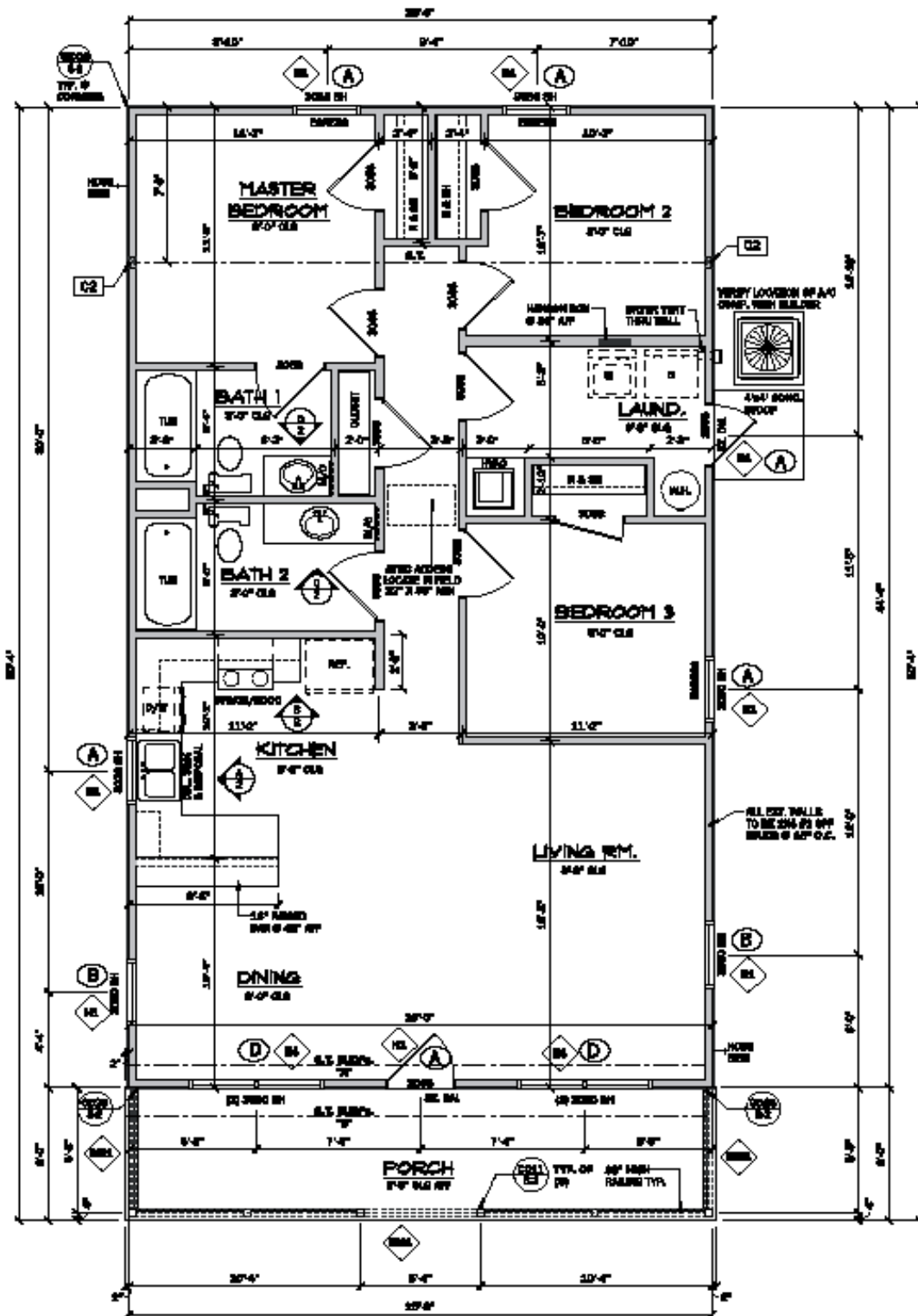
FLOOR PLAN
